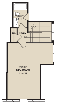
"OPTIONAL" SECOND LEVEL FLOOR PLAN
