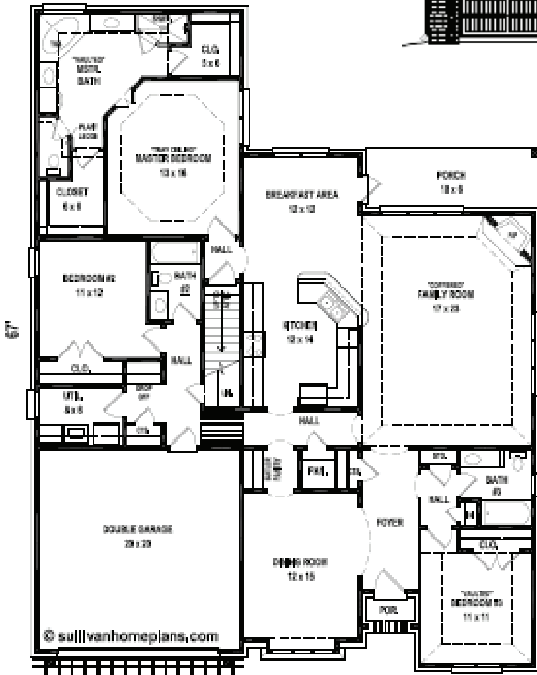
FIRST LEVEL FLOOR PLAN
