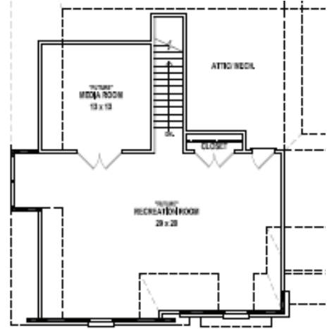
"OPTIONAL" SECOND LEVEL FLOOR PLAN
