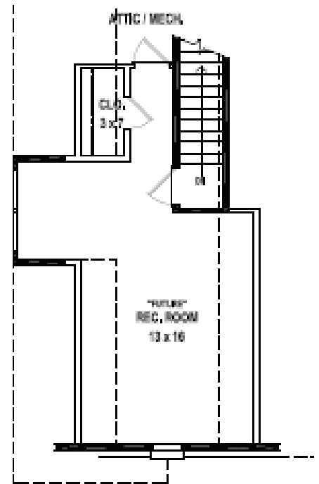
"OPTIONAL" SECOND LEVEL FLOOR PLAN
