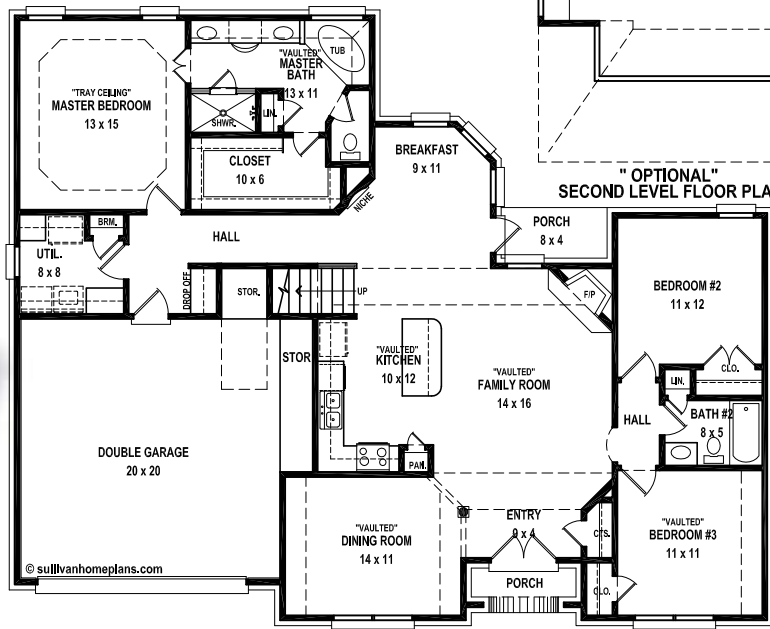
59' FIRST LEVEL FLOOR PLAN
