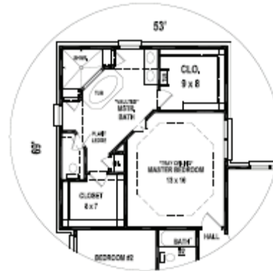
"OPTIONAL" MASTER BATH ADDS 85 SQ. FT. HEATED
